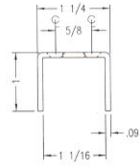
No. 3044 Standard
